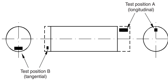
Figure 1 : Plain shaft
