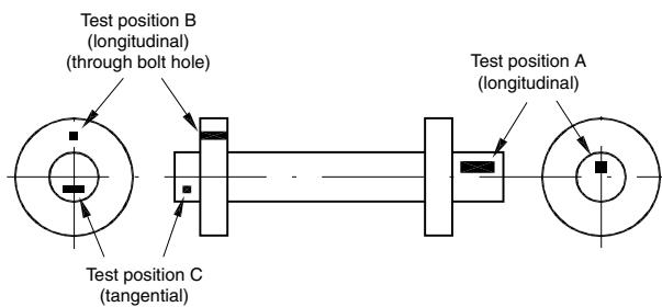
Figure 2 : Flanged shaft
