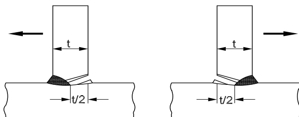
Figure 9 : Break test
