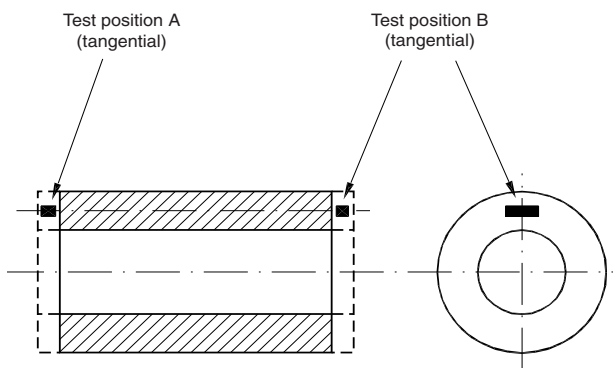
Figure 8 : Pinion sleeve
