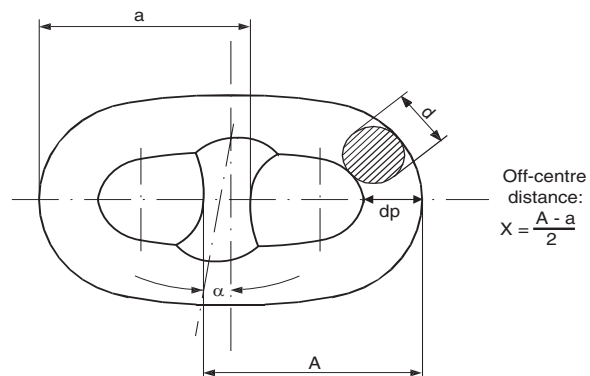
Figure 6 : Manufacturing tolerances
