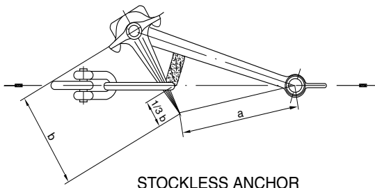
STOCKLESS ANCHOR
