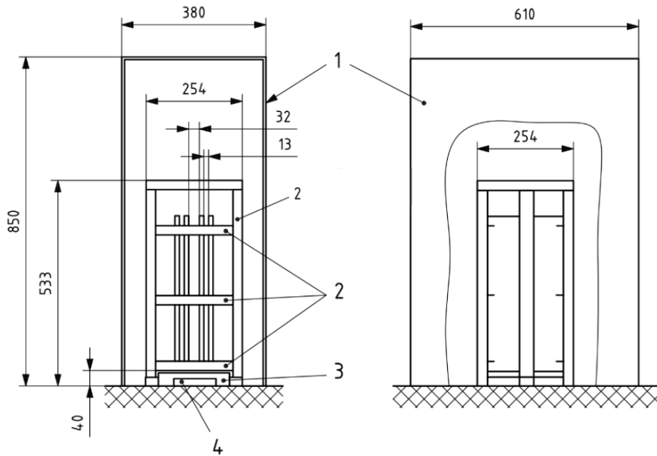
Figure 6: Polymeric sheets fire test arrangement
