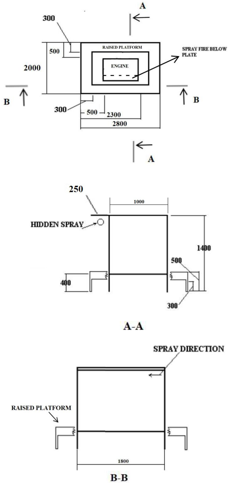
Figure 5: Engine mock-up
