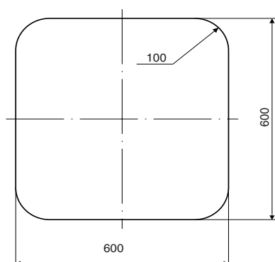
Figure 6 : Minimum horizontal hatch size (1/6/2021)
