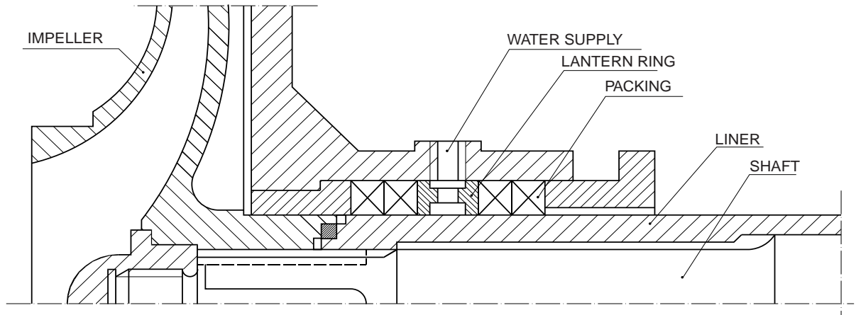
Figure 3 : Seal (1/6/2021)
