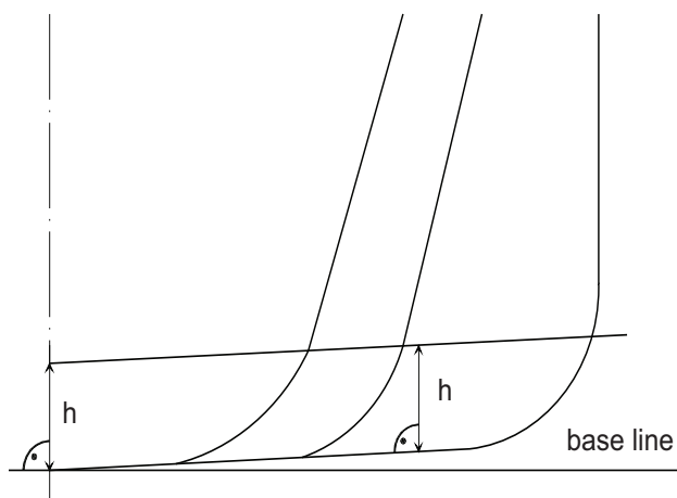
Figure 4 : Cargo tank boundary lines (1/5/2013)
