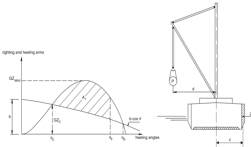
Figure 1 : Cargo lifting (1/7/2014)
