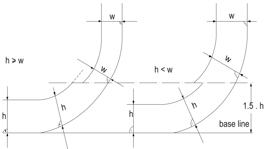
Figure 3 : Cargo tank boundary lines (1/5/2013)
