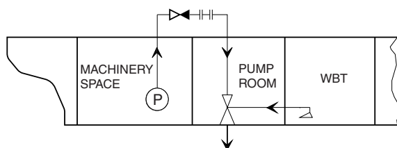
Figure 2 : Discharge arrangement (1/6/2021)
