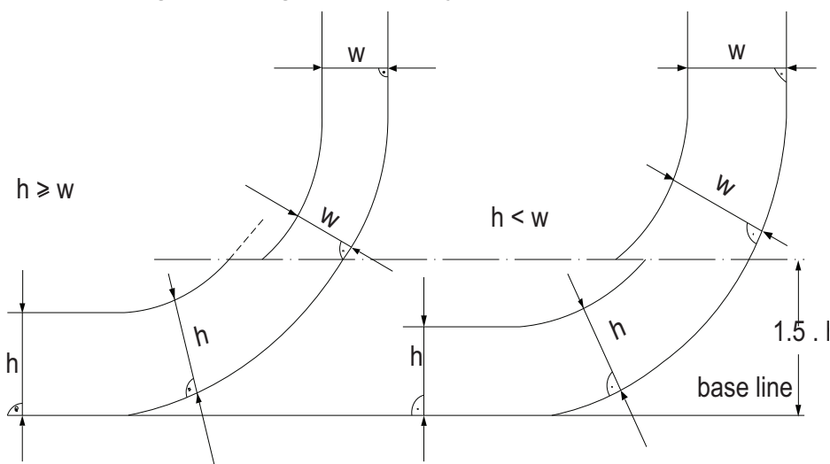
Figure 2 : Cargo tank boundary lines (1/5/2013)
