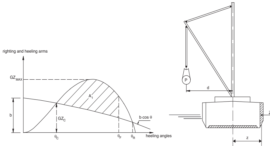
Figure 1 : Cargo lifting
