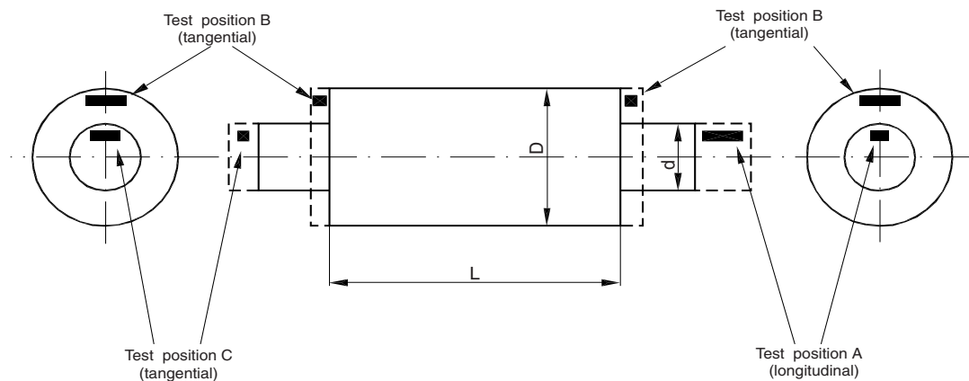
Figure 7 : Pinions
