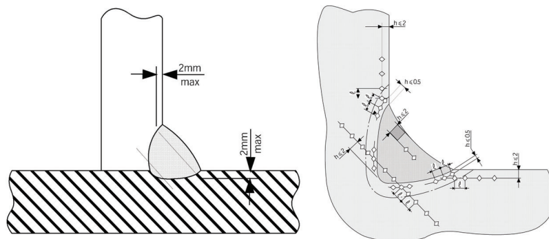
Figure 9 : Macro and hardness indentations (1/1/2015)
