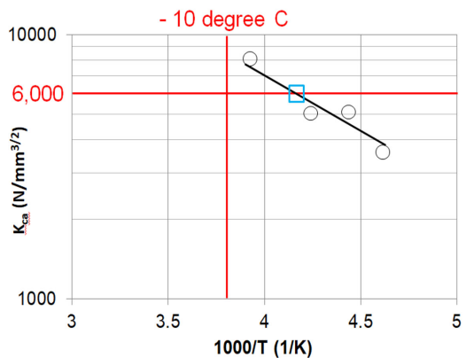
Figure 2 : Example for evaluation of temperature corresponding to the required K_{ca} (1/1/2021)
