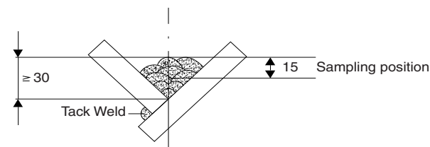
Figure 12 : Deposited weld metal test assembly
