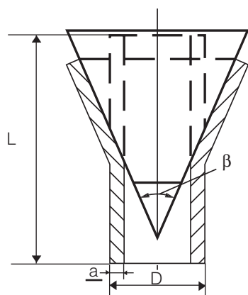
Figure 10 : Drift expanding test (1/7/2004)
