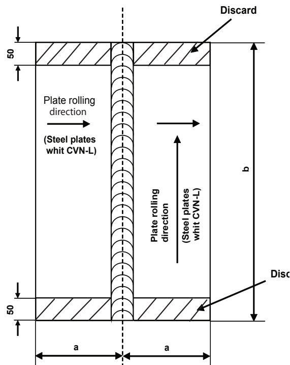
Figure 1 : Plate butt weld test assembly (1/1/2015)
