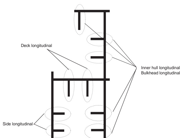
Figure 12 : Upper flange longitudinal structural members (1/1/2014)
