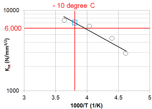
Figure 1 : Example for evaluation of K_{ca} at - 10 degree C (1/1/2021)
