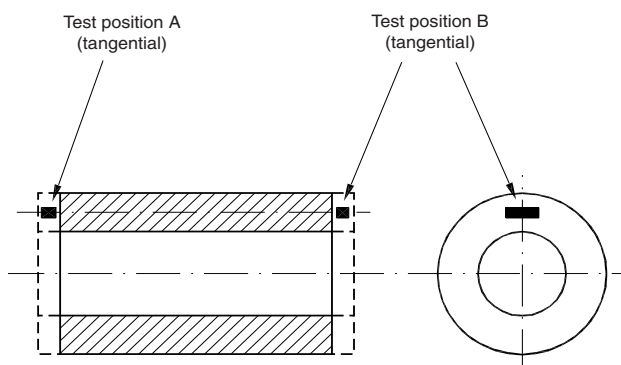
Figure 10 : Pinion sleeve
