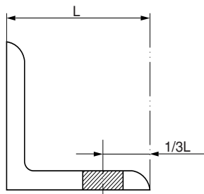
Figure 4 : Angles
