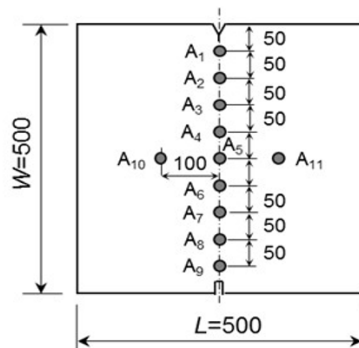
Figure 4 : Locations of temperature measurement (1/1/2021)
