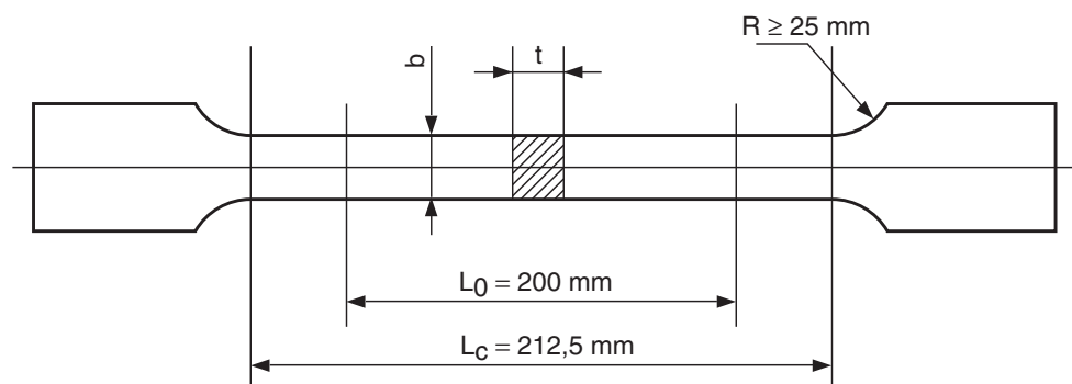
Figure 2 : Non proportional flat specimen (1/7/2004)
