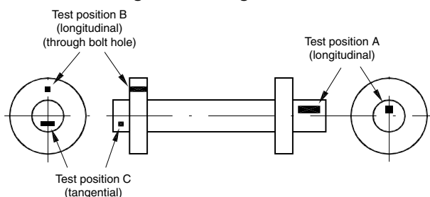
Figure 3 : Flanged shaft
