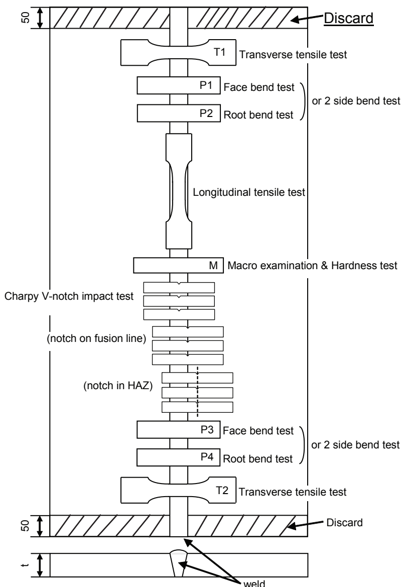
Figure 2 : Location of test specimens (1/1/2015)
