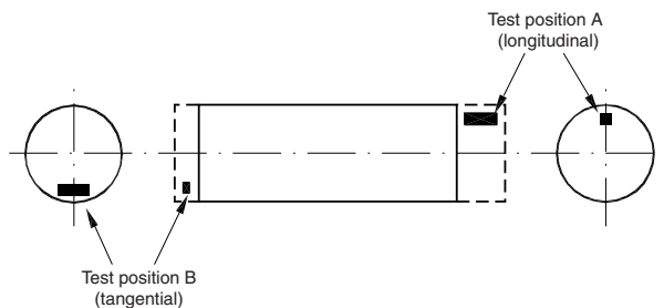
Figure 2 : Plain shaft
