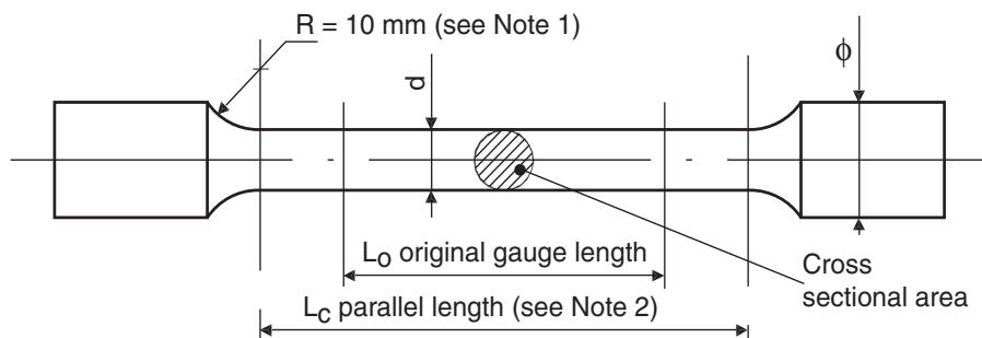
Figure 3 : Round proportional specimen (1/7/2004)
