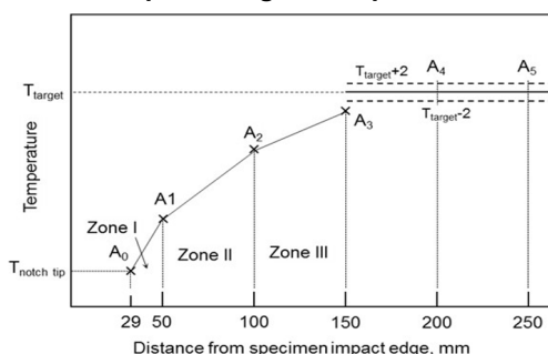
Figure 6 : Schematic temperature gradient profile in LTG zone (1/1/2021)
